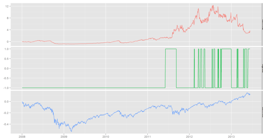
Figure 8. Equity line and signal of II strategy for VIX index futures and S&P500 index.
